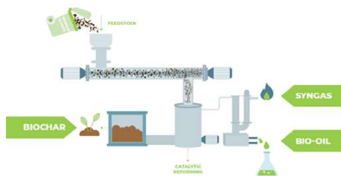
Process flow diagram. Credit: To-Syn-Fuel project.
